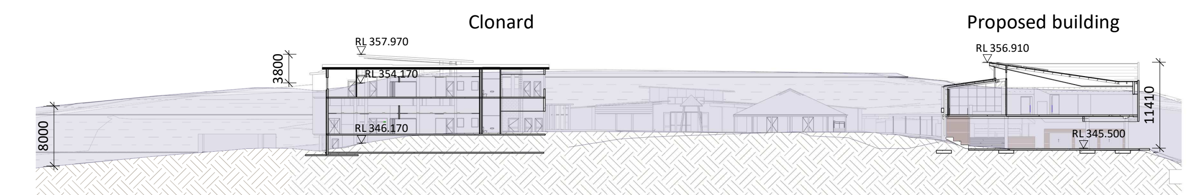
4 Section 4 - Height Analysis 1 : 500
