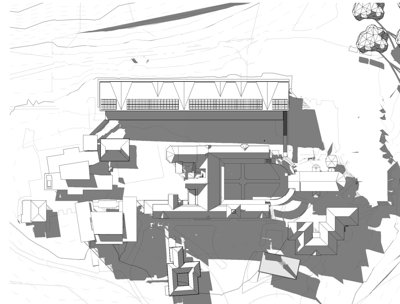
6 21st June 3pm 1 : 1500
